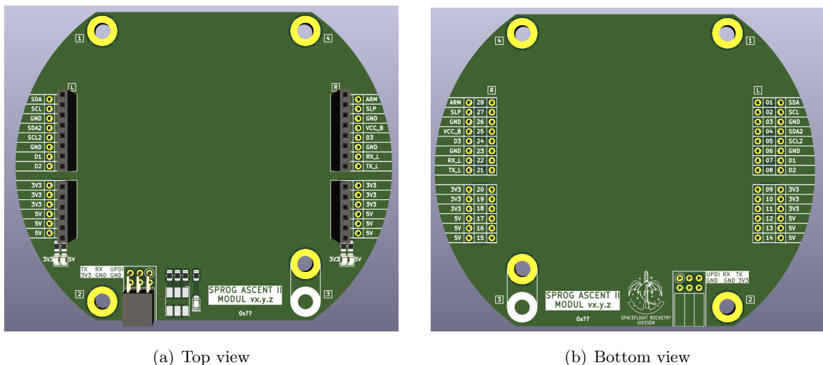
Figure 5.1.2: PCB concept
