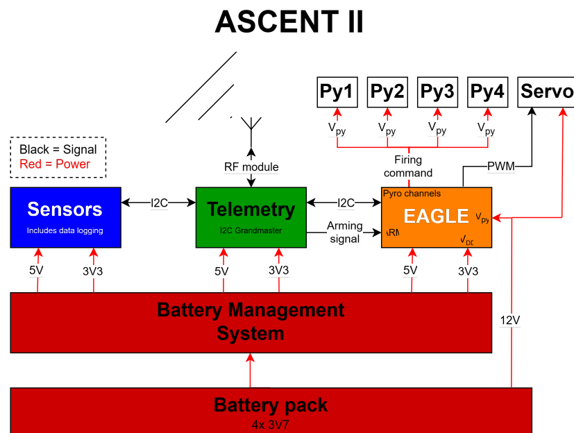
Figure 5.1.1: ASCENT II architecture
