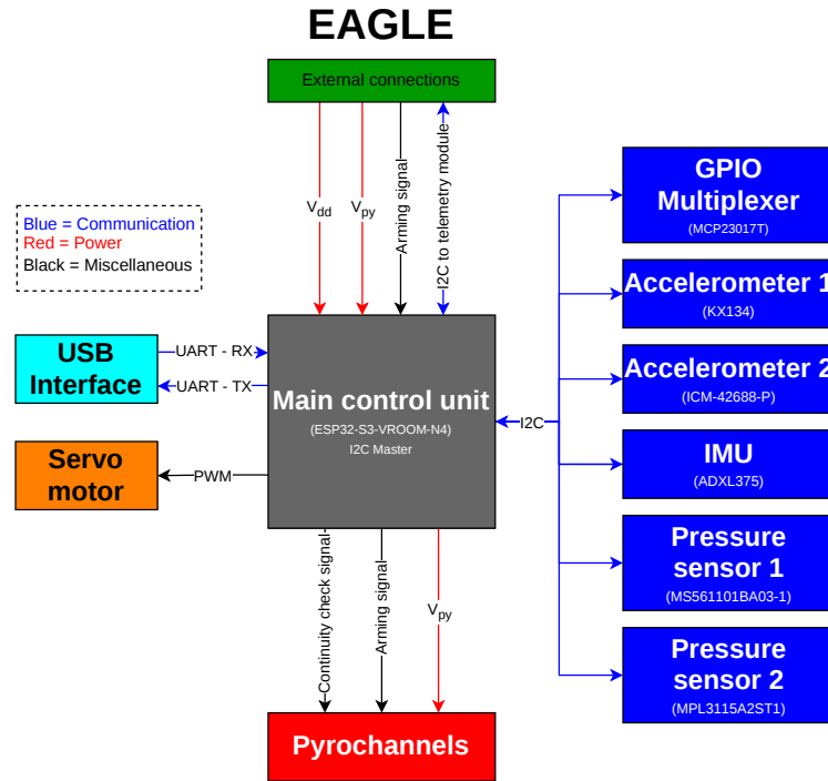
Figure 5.1.3: EAGLE architecture
