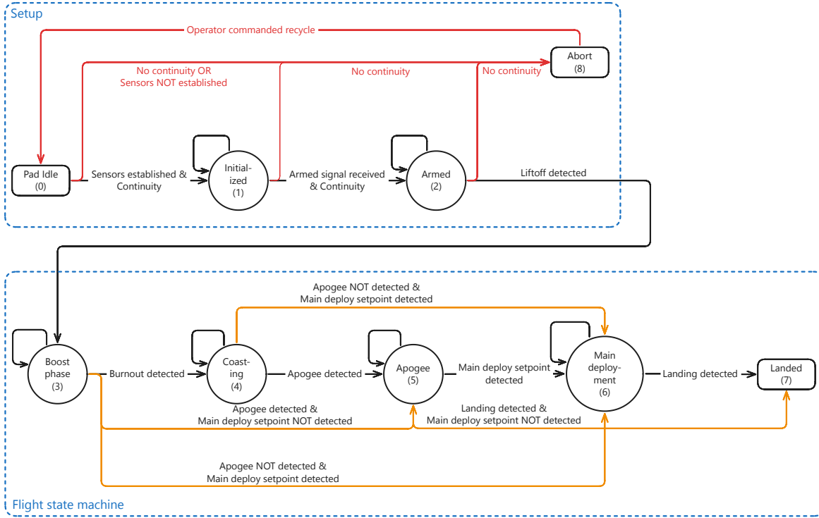
Figure 5.2.1: Software architecture
